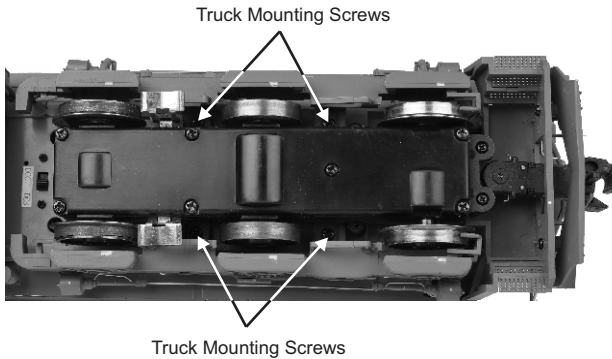
Figure: Truckside Mounting Screw Locations
