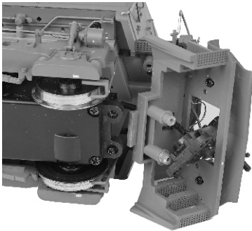
Figure: Pilot Removed and the Coupler Unattached
