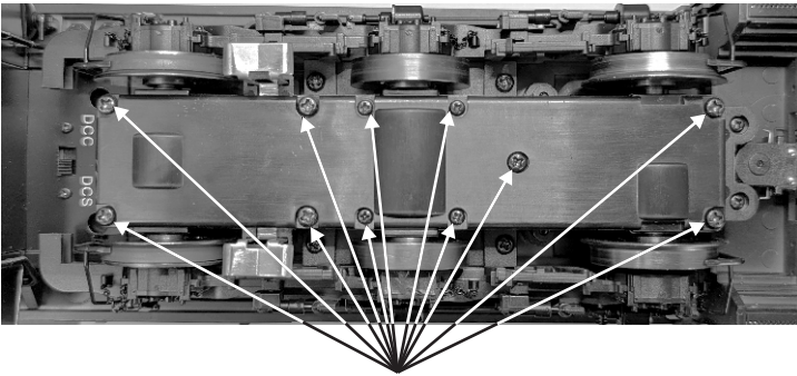
Remove (11) Gear Box Cover Screws
