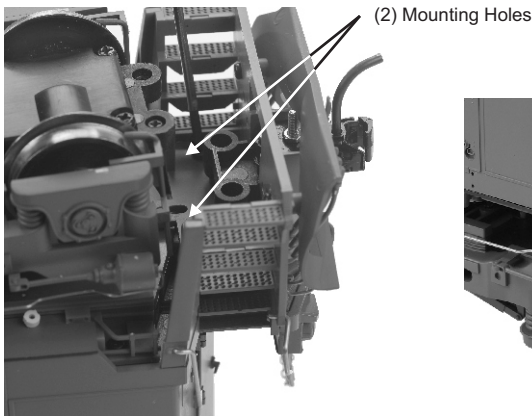
Figure: The fixed pilot mounts to the body by these mounting holes.
