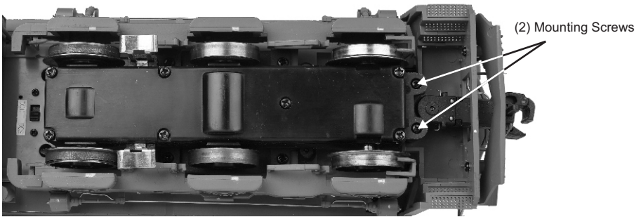
Figure: Mounting Screw Locations
