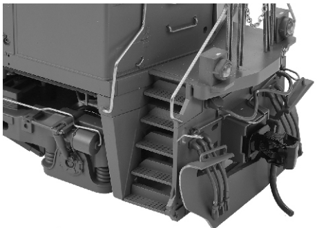
Figure: Fixed Pilot Mounted to Chassis
