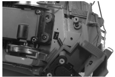
Figure: The PS3 Coupler Connector Must Be Unplugged
