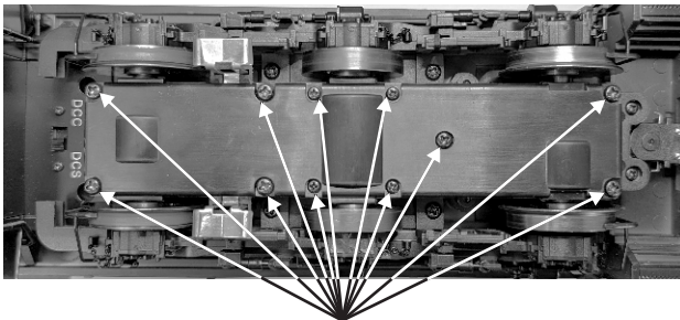
Remove (11) Gear Box Mount Screws
