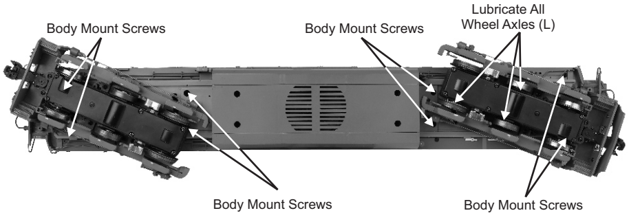
Figure: Body Mount Screws and Lubrication Points on the Locomotive
